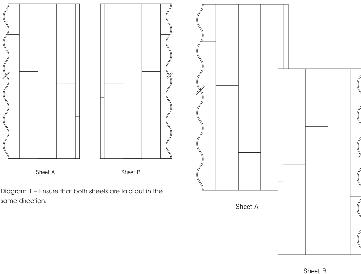
Diagram 2 – Both edges of the sheet have a narrow edge which needs to be trimmed to leave a full plank. Overlap sheet A over sheet B as indicated above and cut in the joint, cutting both sheets so that the join runs down the edge of the planks.
